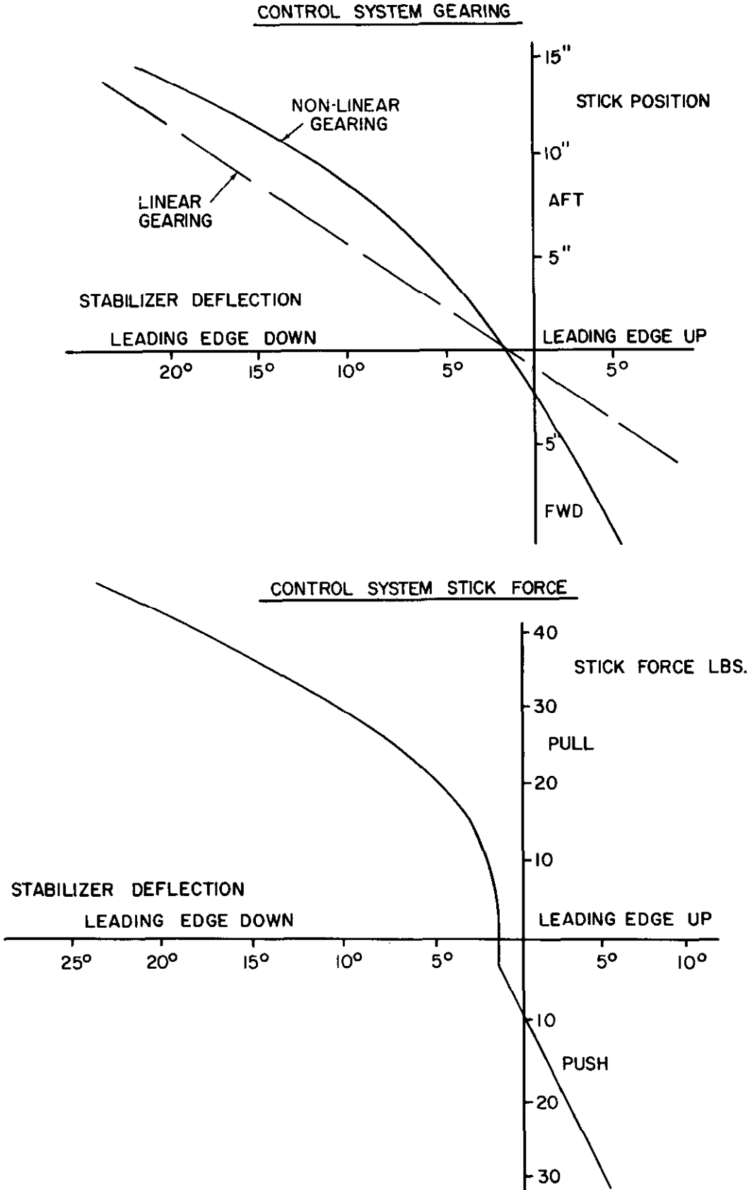
Figure 4.21. Longitudinal Control System
