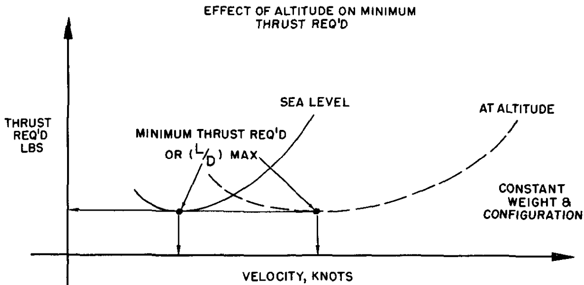
Figure 2.27. Endurance Performance
