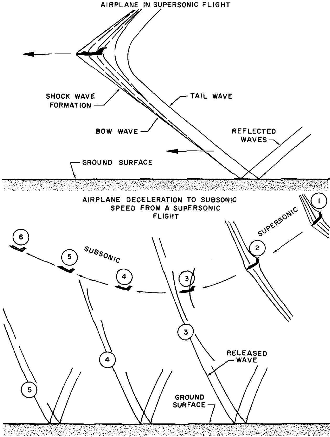
Figure 6.14. Sonic Booms
