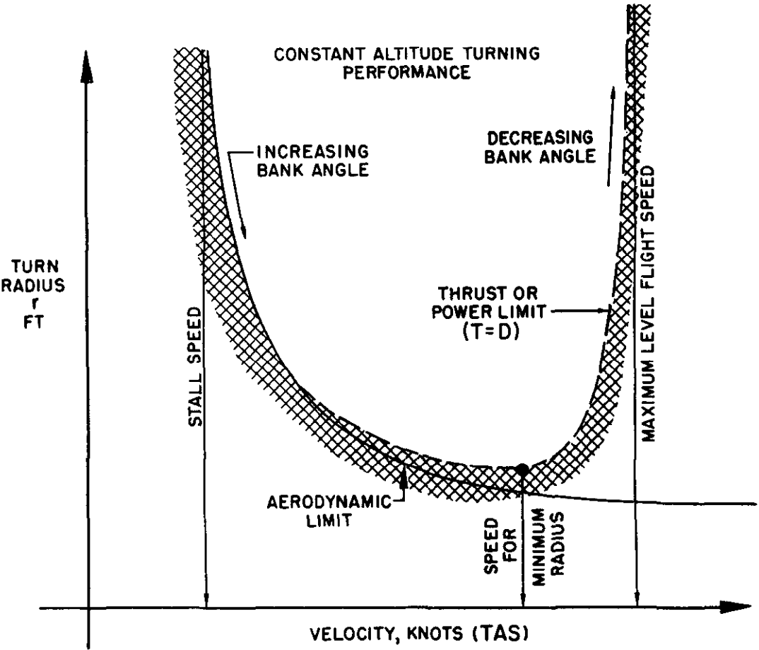
Figure 2.30. Maneuvering Performance
