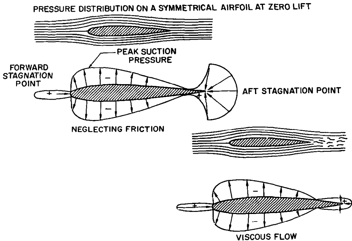
Figure 1.7. Streamline Pattern and Pressure Distribution
