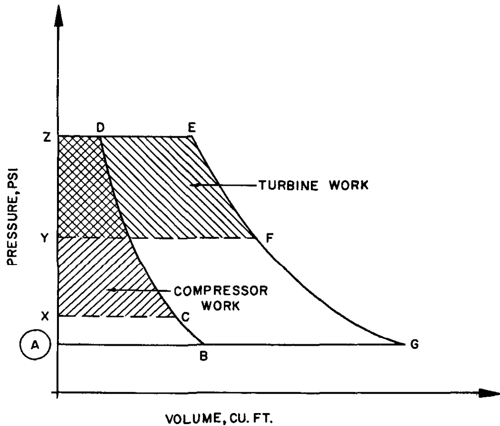
Figure 2.6. Turbojet Engines
