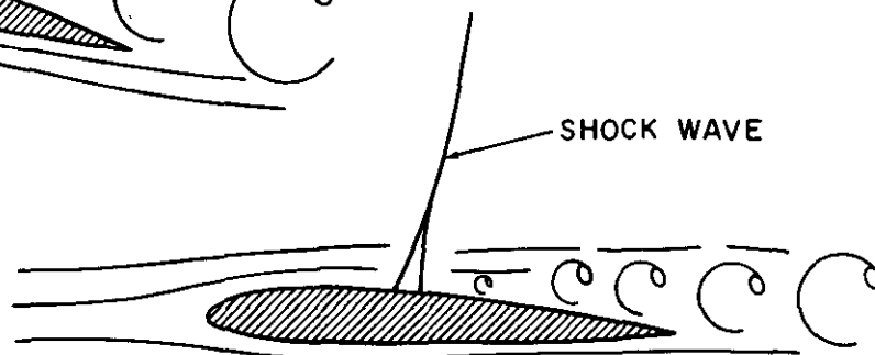
SHOCK WAVE INDUCED FLOW SEPARATION
