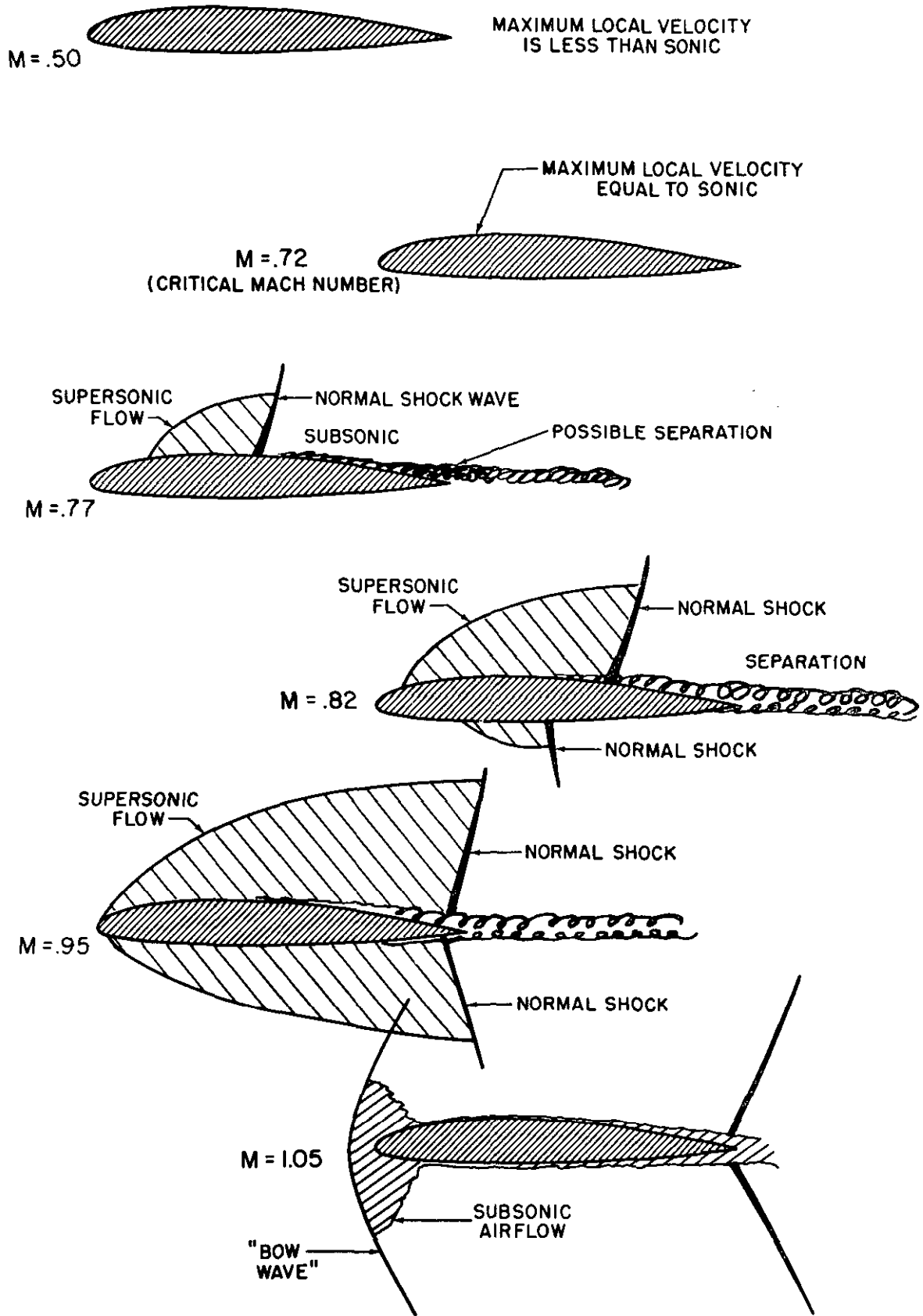
Figure 3.9. Transonic Flow Patterns (sheet 1 of 2)
